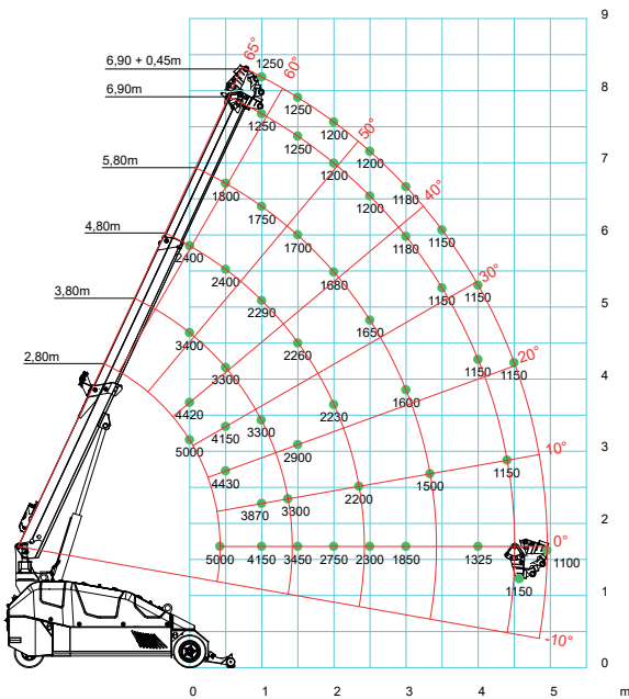
Hook Load Chart
